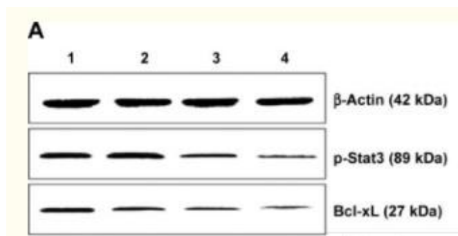
Western Blot analysis of various cells using Bcl-x Monoclonal Antibody
