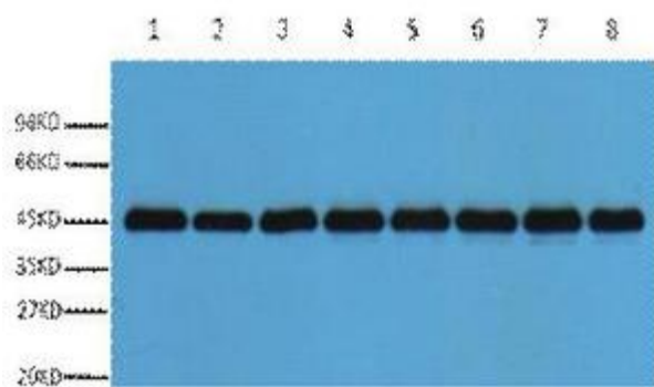
Western Blot analysis of various cells using Plant-actin Monoclonal Antibody
