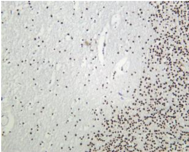
Human brain was stained with anti-Histone H3 (Tri Methyl Lys79) Rabbit antibody
