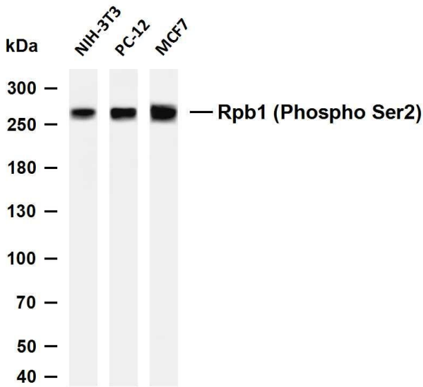
Various whole cell lysates were separated by 4-8% SDS-PAGE, and the membrane was blotted with anti-Rpb1 (Phospho Ser2) antibody. The HRP-conjugated Goat anti-Rabbit IgG (H + L) antibody was used to detect the antibody. Lane 1: NIH-3T3 Lane 2: PC-12 Lane 3: MCF7 Predicted band size: 217kDa Observed band size: 270kDa
