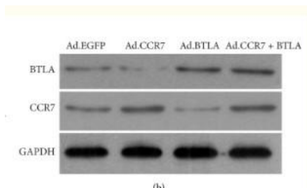
Western Blot analysis of various cells using CD272 Monoclonal Antibody
