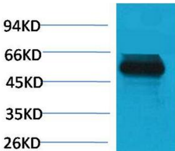
Western Blot analysis of various cells using TRIM72 Monoclonal Antibody
